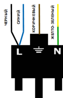
PROMATIC DURAPLUG
